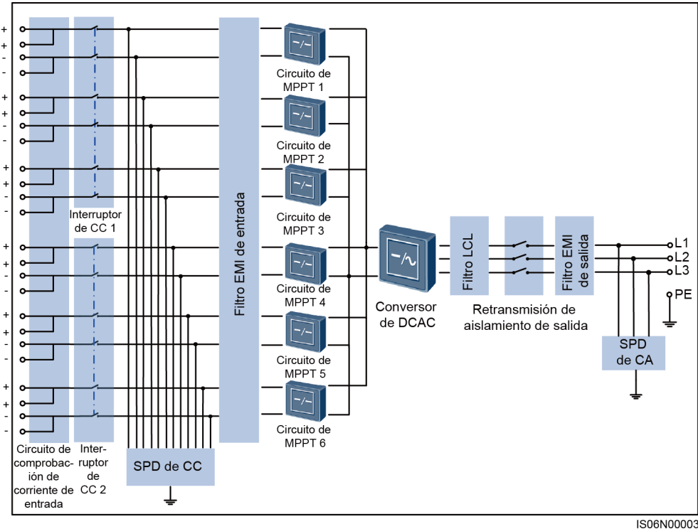
Figura 2-6 Diagrama conceptual del SUN2000-65KTL-M0
