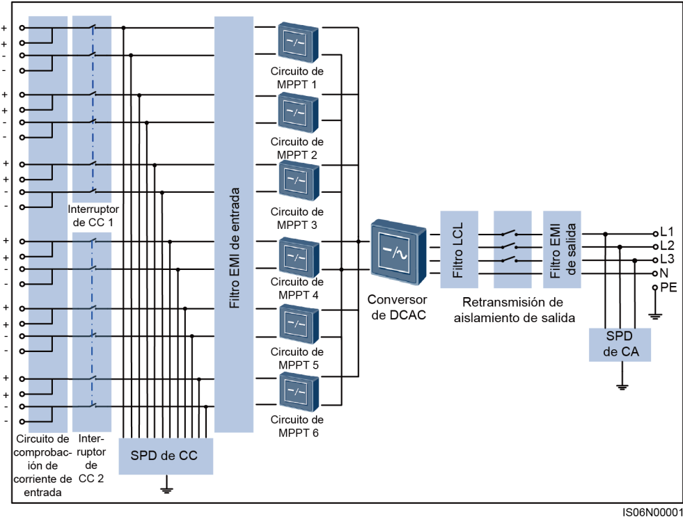
Figura 2-5 Diagrama conceptual del SUN2000-50KTL/60KTL-M0
