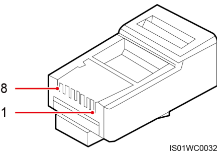
Figura 5-29 conector RJ45
